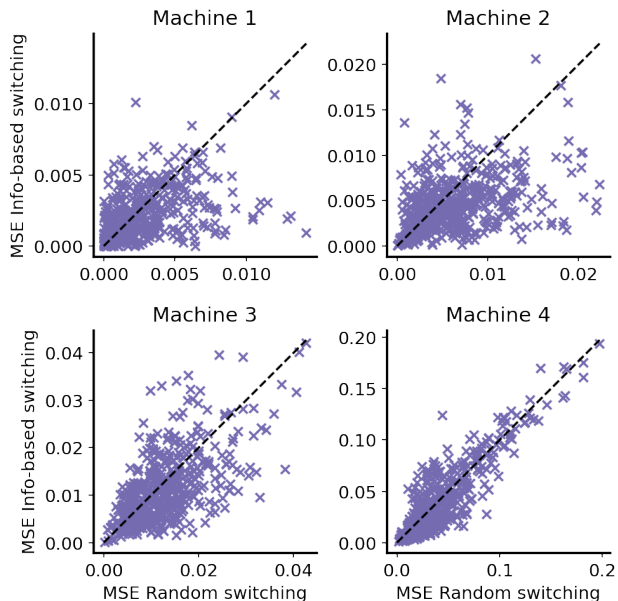
Figure 4: Comparison of information-based vs. random switching on the MIMII dataset. Under the line is better for MF-BOCD. See Table 1 for means and standard errors.
