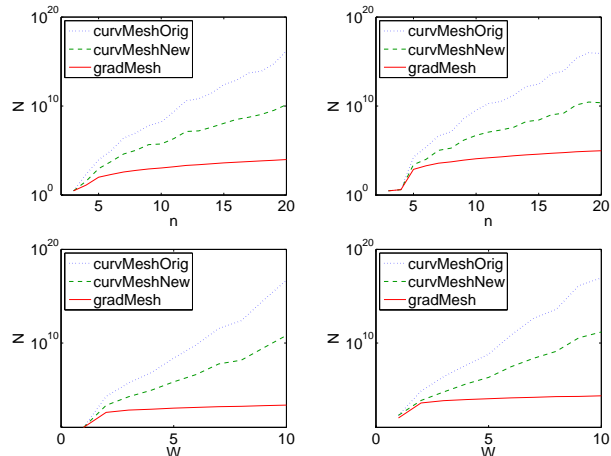
Figure 2: Variation in N = sum of number of mesh points in each dimension, log scale , as: (top) n = number of variables is changed, keeping W = 5 fixed; (bottom) W = maximum coupling strength is changed, keeping n = 10 fixed. On the left, \epsilon = 1 (medium resolution); on the right, \epsilon = 0.1 (fine resolution). In each case the topology is a complete graph, edge weights are chosen W_{ij} \sim U[-W, W] and \theta_i \sim U[-2, 2] . Average over 10 random models for each value. curvMeshOrig is the original method of Weller and Jebara (2013a); curvMeshNew is our refinement, see §4; gradMesh is our new first derivative minsum method, see §3. For more details, see text of §6.1.
